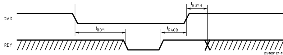
FIGURE 10. Ready Feedback Timing Diagram
